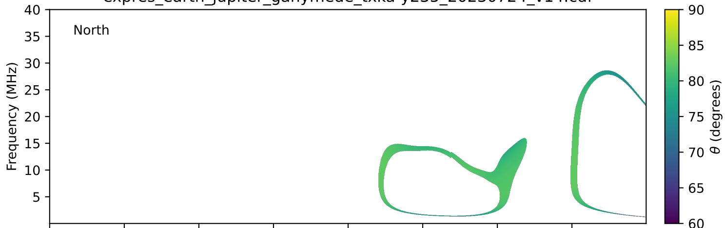
expres_earth_jupiter_ganymede_txka-y235_20230724_v14.cdf
