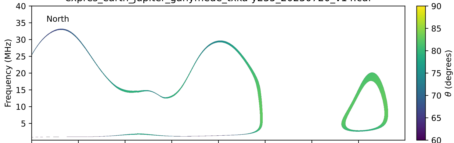
expres_earth_jupiter_ganymede_txka-y235_20230720_v14.cdf
