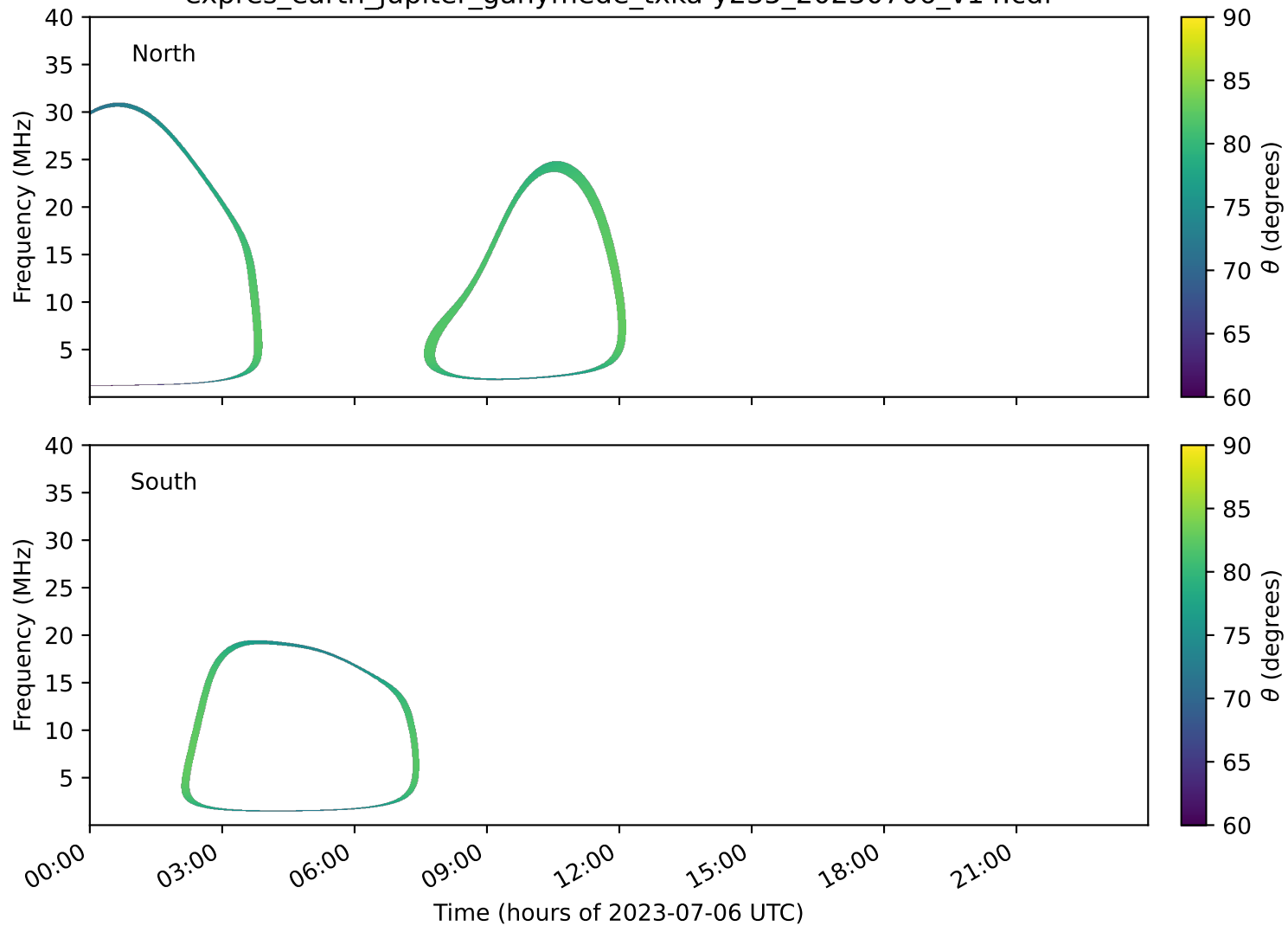
expres_earth_jupiter_ganymede_txka-y235_20230706_v14.cdf
