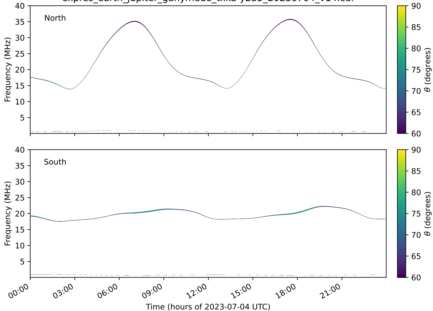
expres_earth_jupiter_ganymede_txka-y235_20230704_v14.cdf
