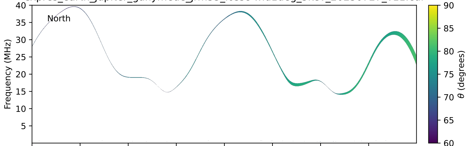
expres_earth_jupiter_ganymede_jrm33_lossc-wid1deg_3kev_20230727_v11.cdf
