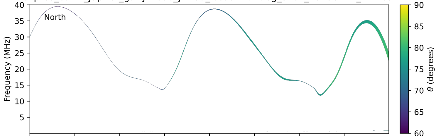
expres_earth_jupiter_ganymede_jrm09_lossc-wid1deg_3kev_20230727_v11.cdf
