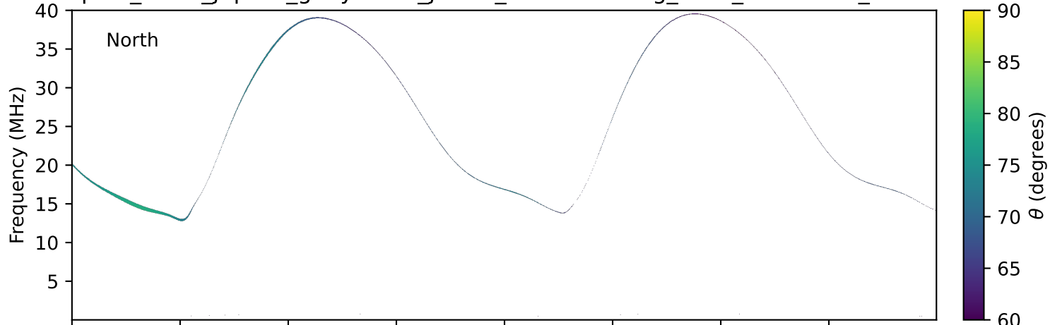
expres_earth_jupiter_ganymede_jrm09_lossc-wid1deg_3kev_20230711_v11.cdf
