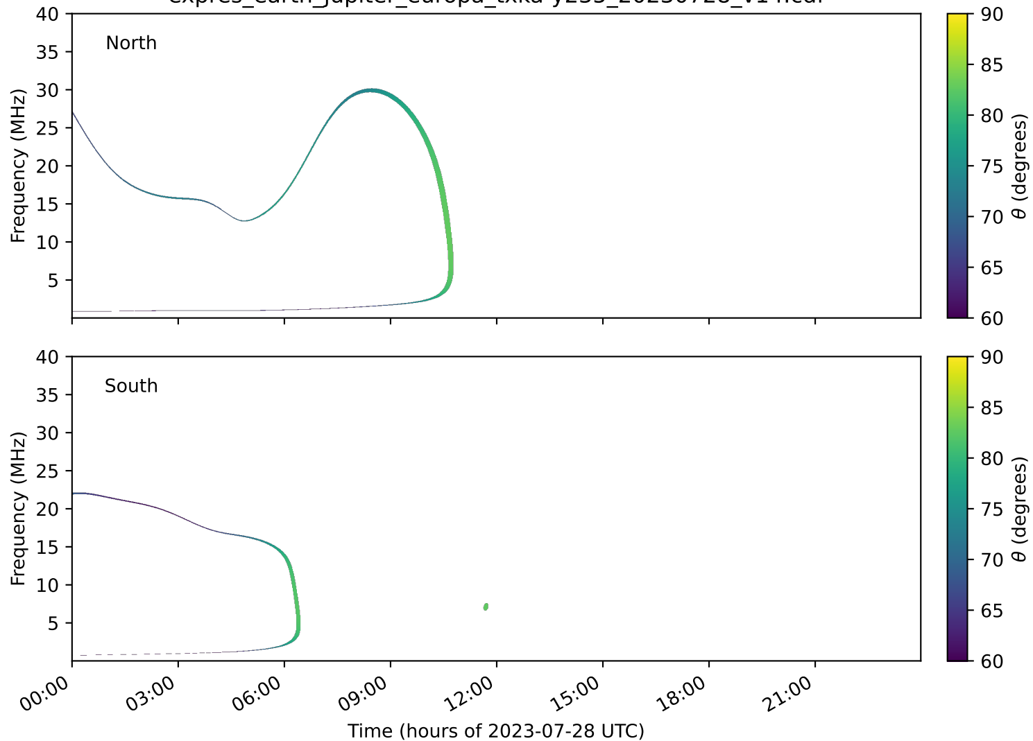
expres_earth_jupiter_europa_txka-y235_20230728_v14.cdf
