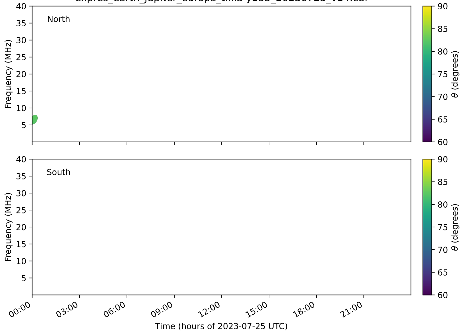
expres_earth_jupiter_europa_txka-y235_20230725_v14.cdf
