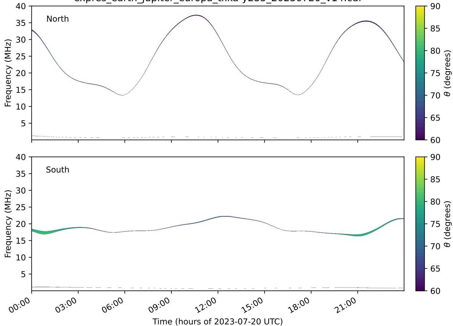
expres_earth_jupiter_europa_txka-y235_20230720_v14.cdf
