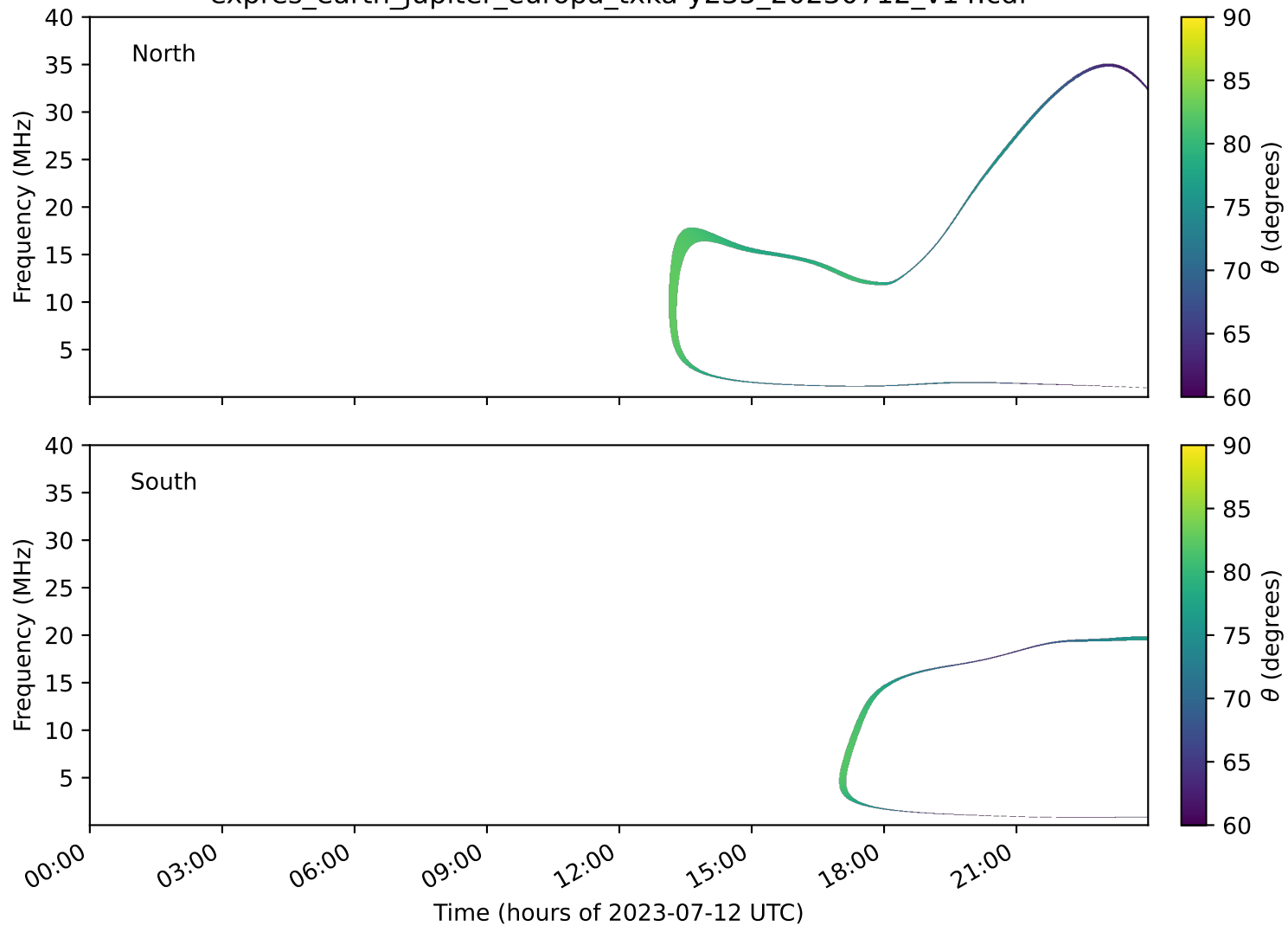
expres_earth_jupiter_europa_txka-y235_20230712_v14.cdf
