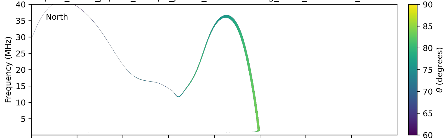
expres_earth_jupiter_europa_jrm09_lossc-wid1deg_3kev_20230703_v11.cdf
