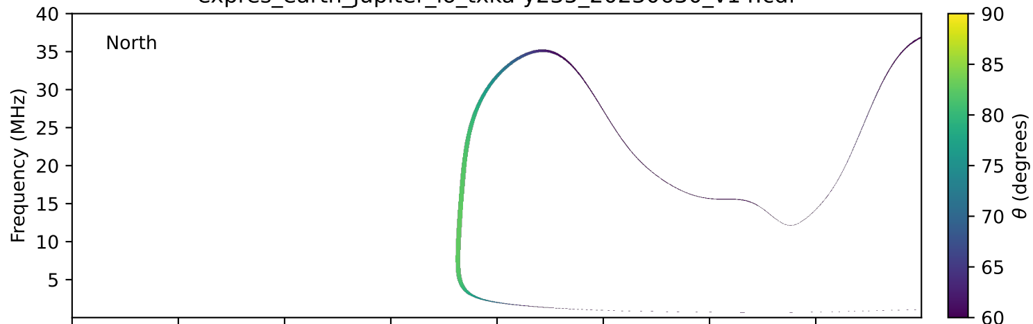
expres_earth_jupiter_io_txka-y235_20230630_v14.cdf
