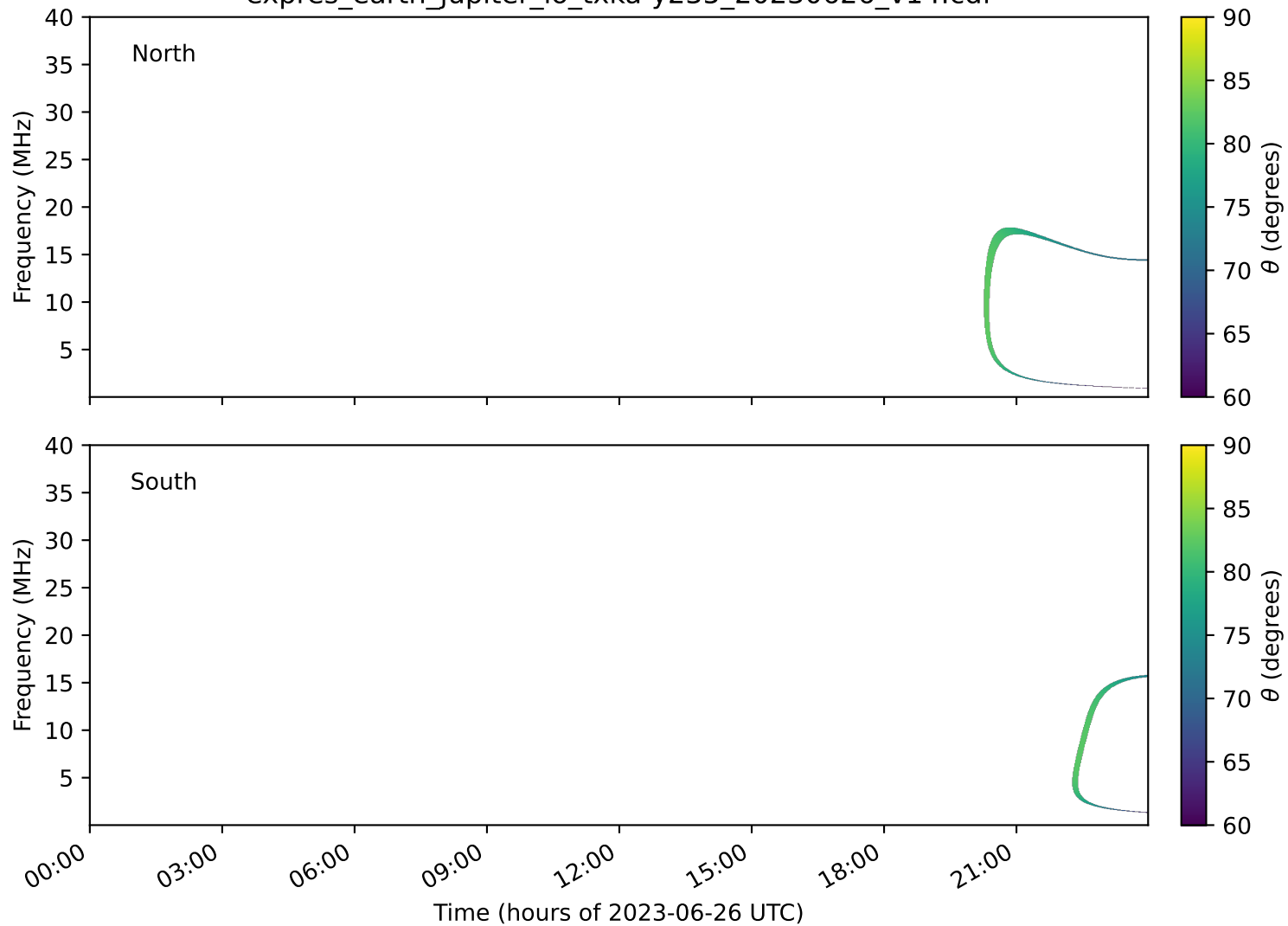
expres_earth_jupiter_io_txka-y235_20230626_v14.cdf
