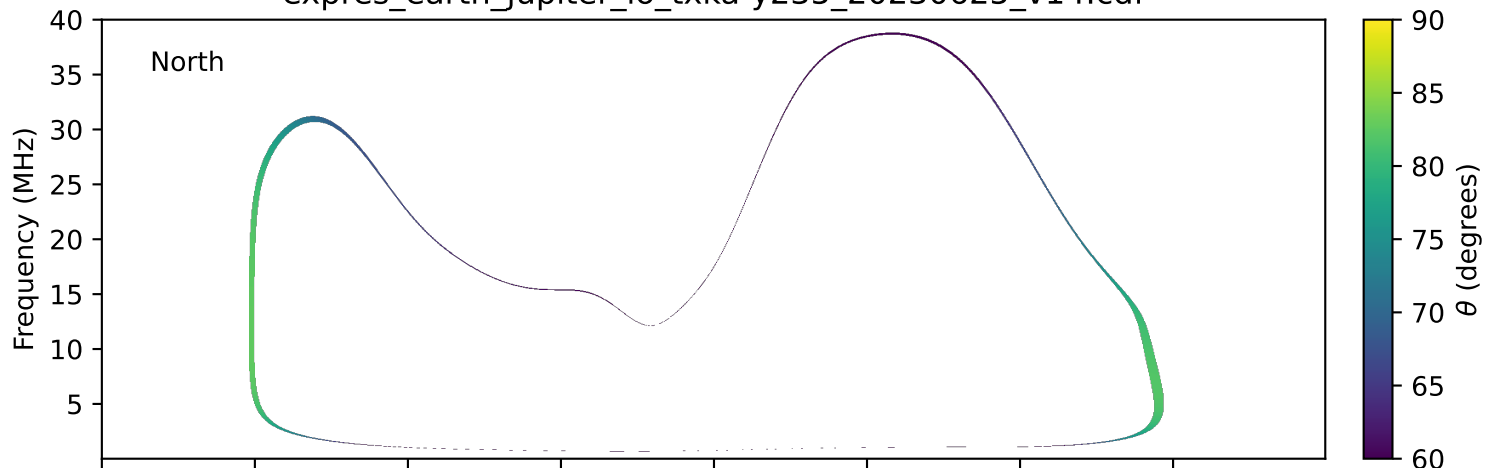
expres_earth_jupiter_io_txka-y235_20230625_v14.cdf
