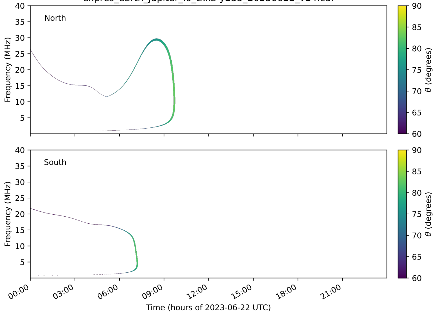
expres_earth_jupiter_io_txka-y235_20230622_v14.cdf
