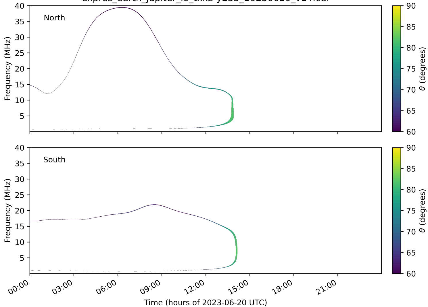
expres_earth_jupiter_io_txka-y235_20230620_v14.cdf
