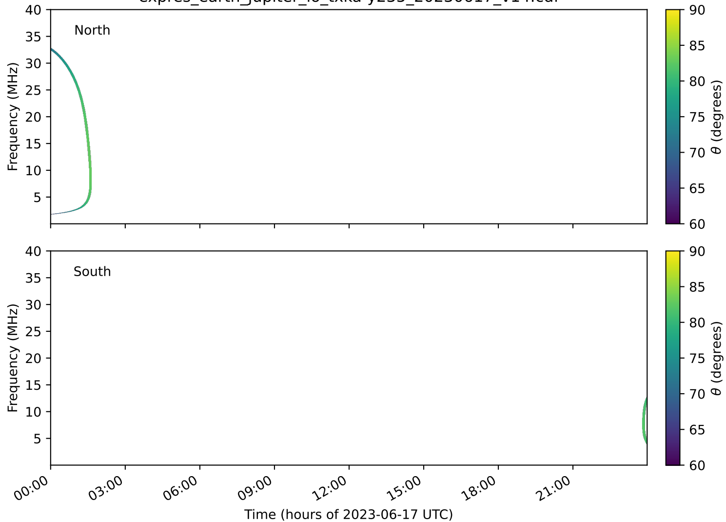
expres_earth_jupiter_io_txka-y235_20230617_v14.cdf
