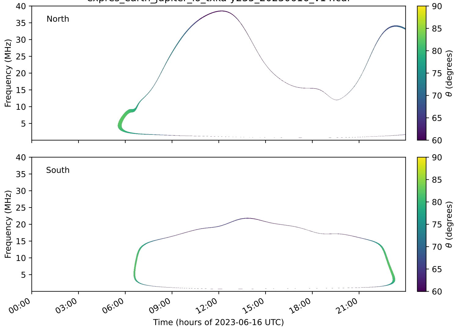
expres_earth_jupiter_io_txka-y235_20230616_v14.cdf
