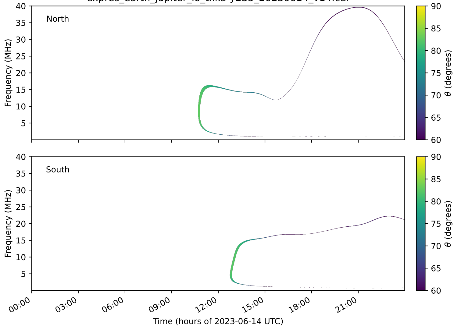
expres_earth_jupiter_io_txka-y235_20230614_v14.cdf
