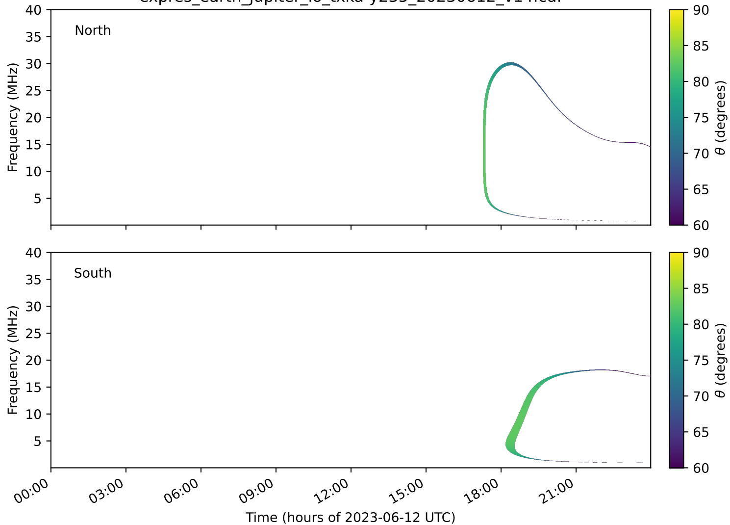
expres_earth_jupiter_io_txka-y235_20230612_v14.cdf
