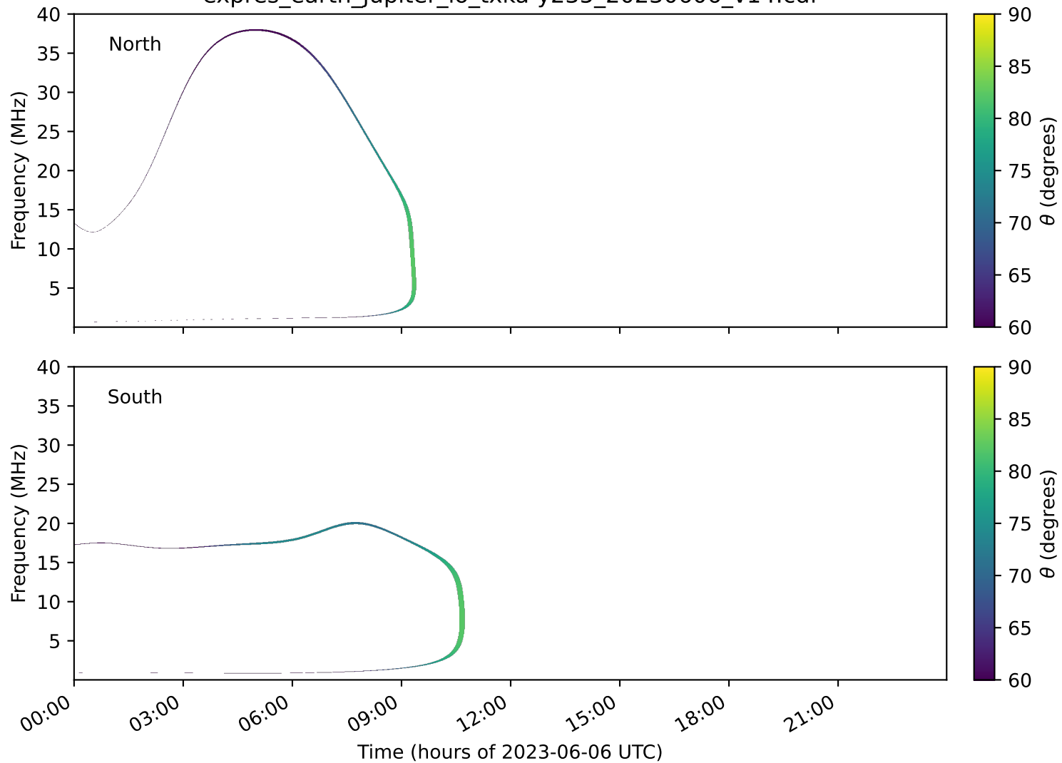
expres_earth_jupiter_io_txka-y235_20230606_v14.cdf
