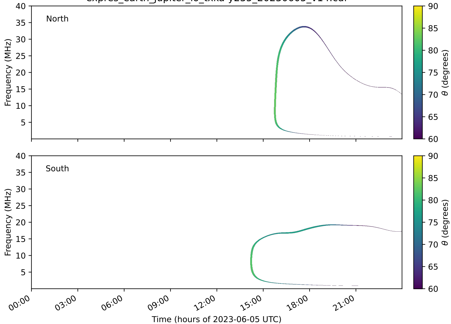
expres_earth_jupiter_io_txka-y235_20230605_v14.cdf
