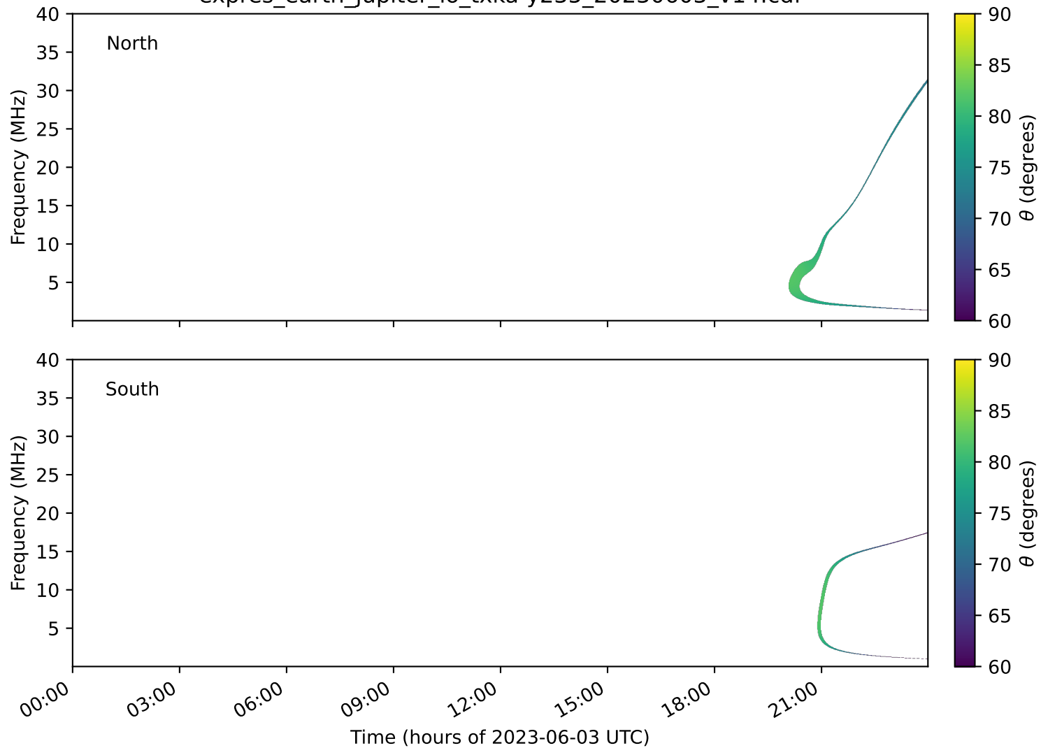
expres_earth_jupiter_io_txka-y235_20230603_v14.cdf
