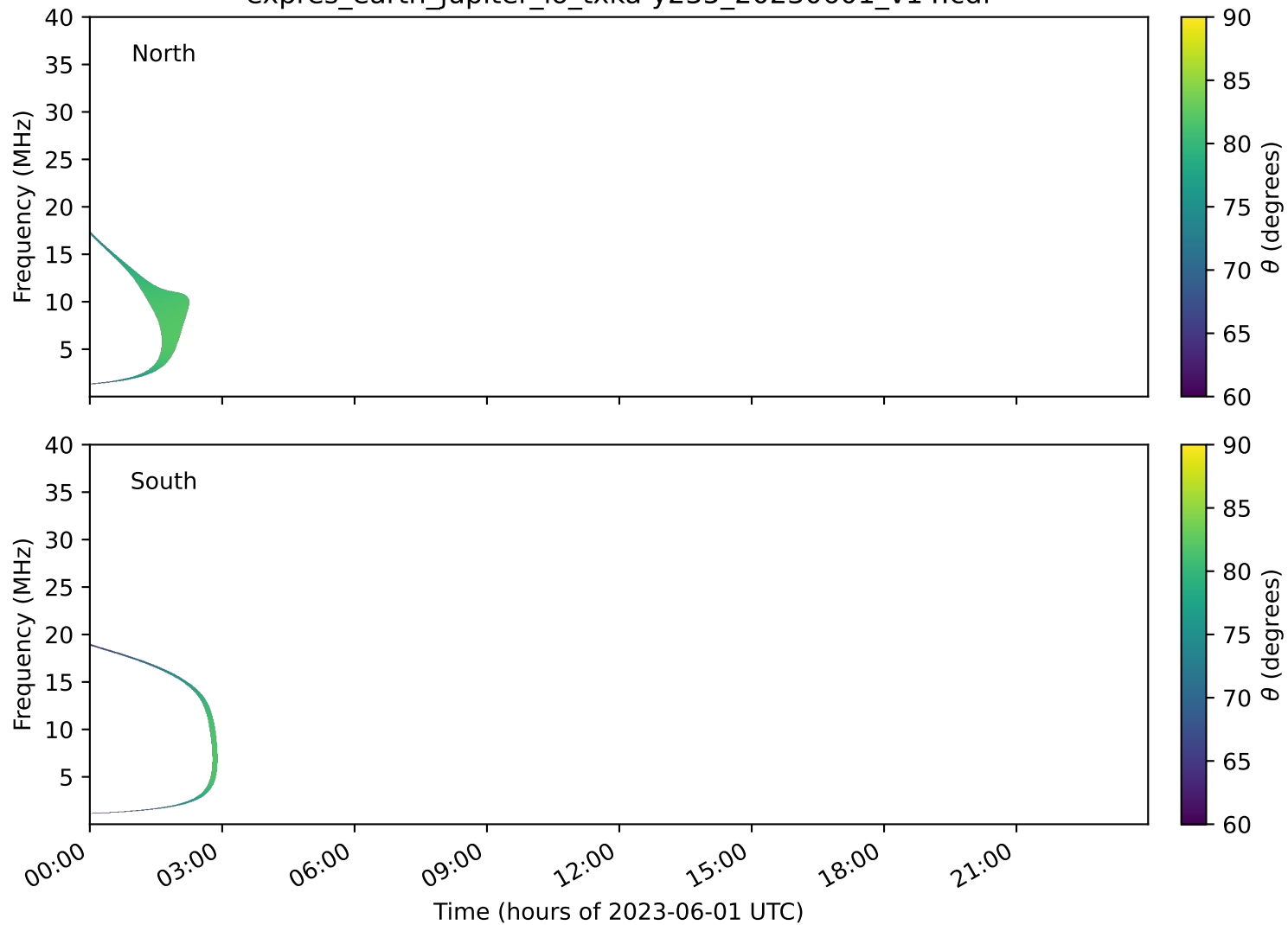
expres_earth_jupiter_io_txka-y235_20230601_v14.cdf
