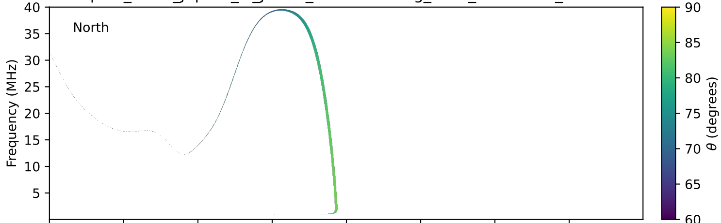
expres_earth_jupiter_io_jrm33_lossc-wid1deg_3kev_20230629_v11.cdf
