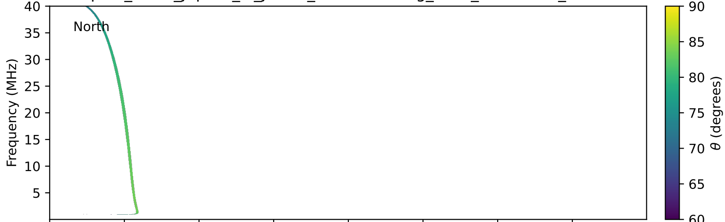
expres_earth_jupiter_io_jrm33_lossc-wid1deg_3kev_20230624_v11.cdf
