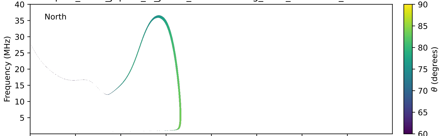
expres_earth_jupiter_io_jrm33_lossc-wid1deg_3kev_20230622_v11.cdf
