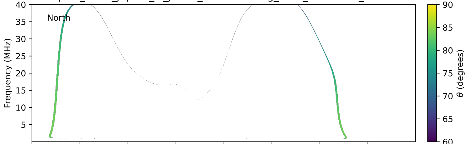
expres_earth_jupiter_io_jrm33_lossc-wid1deg_3kev_20230618_v11.cdf
