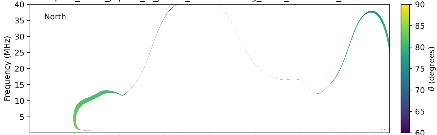
expres_earth_jupiter_io_jrm33_lossc-wid1deg_3kev_20230609_v11.cdf
