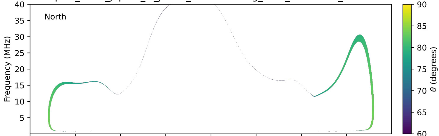
expres_earth_jupiter_io_jrm33_lossc-wid1deg_3kev_20230602_v11.cdf
