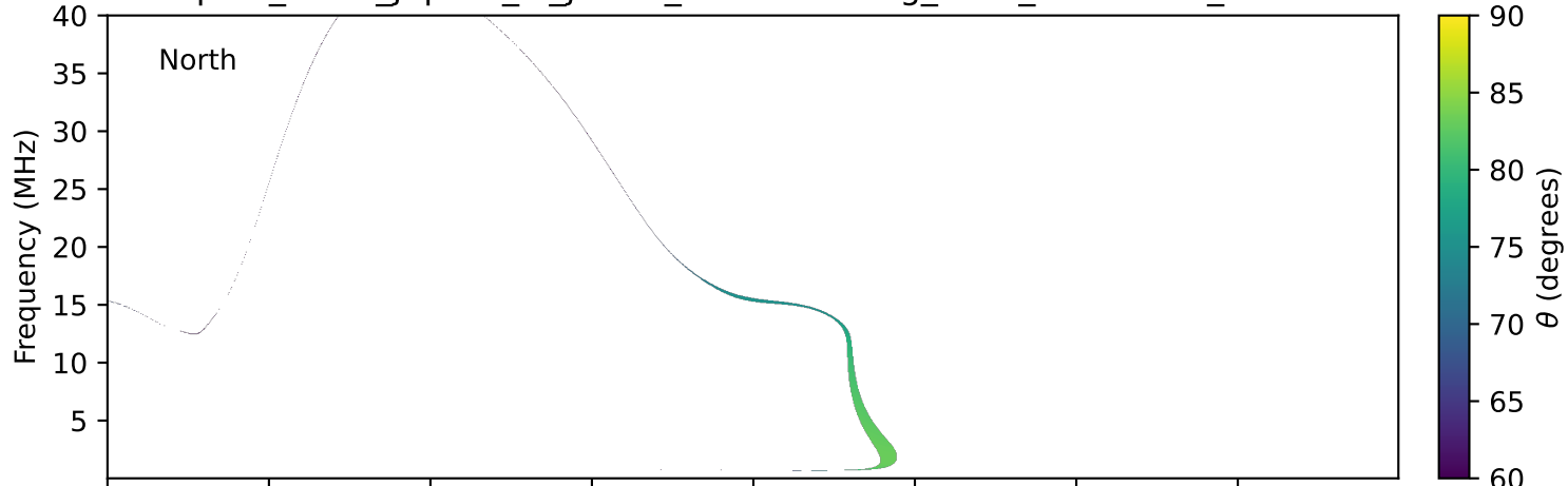
expres_earth_jupiter_io_jrm09_lossc-wid1deg_3kev_20230620_v11.cdf
