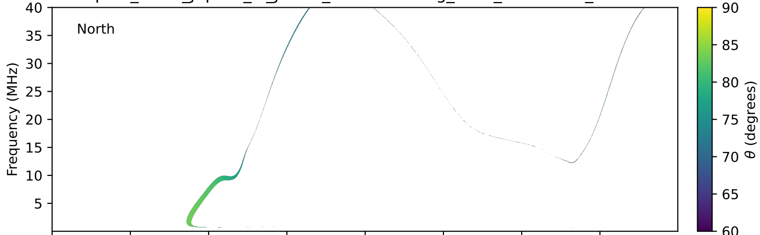
expres_earth_jupiter_io_jrm09_lossc-wid1deg_3kev_20230616_v11.cdf
