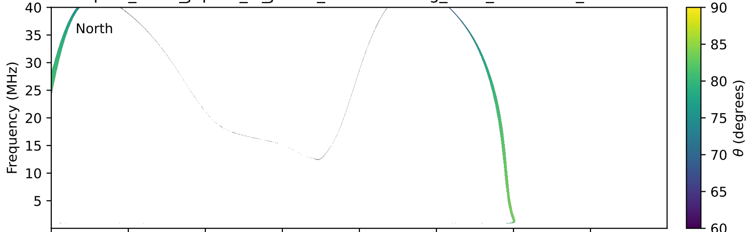
expres_earth_jupiter_io_jrm09_lossc-wid1deg_3kev_20230611_v11.cdf
