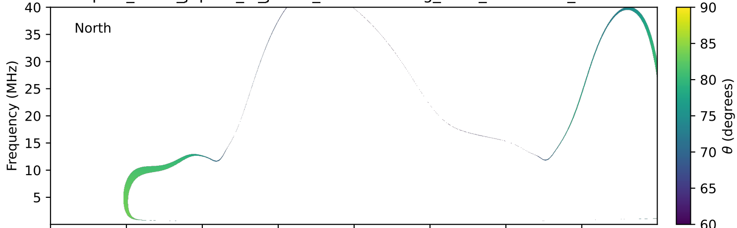
expres_earth_jupiter_io_jrm09_lossc-wid1deg_3kev_20230609_v11.cdf
