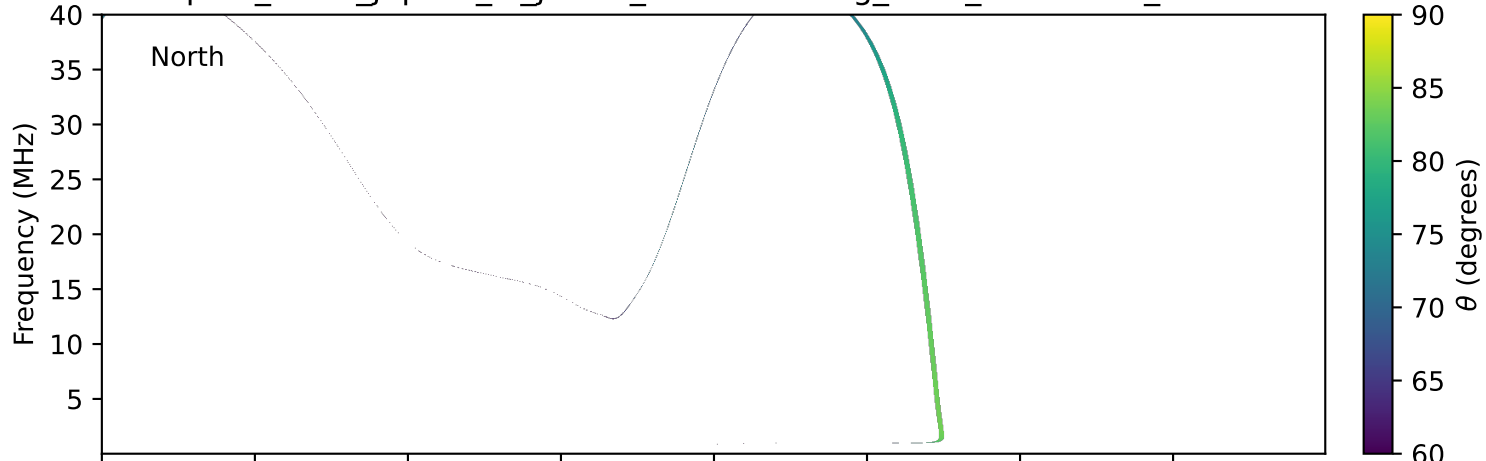
expres_earth_jupiter_io_jrm09_lossc-wid1deg_3kev_20230604_v11.cdf
