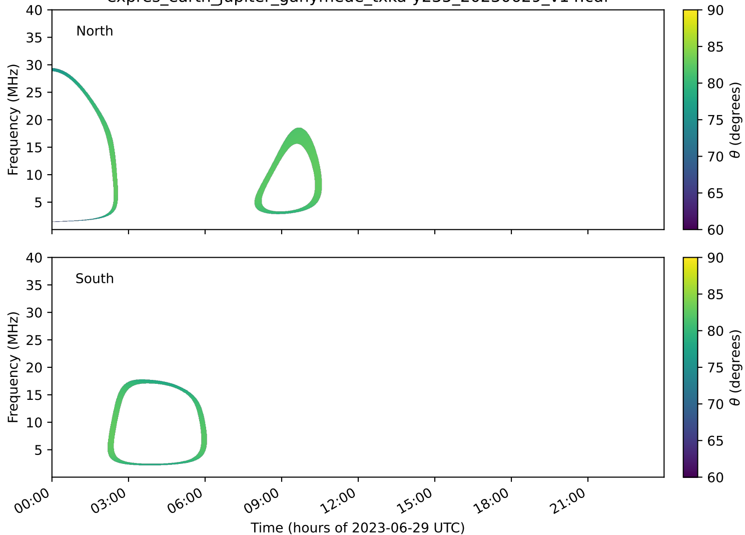
expres_earth_jupiter_ganymede_txka-y235_20230629_v14.cdf
