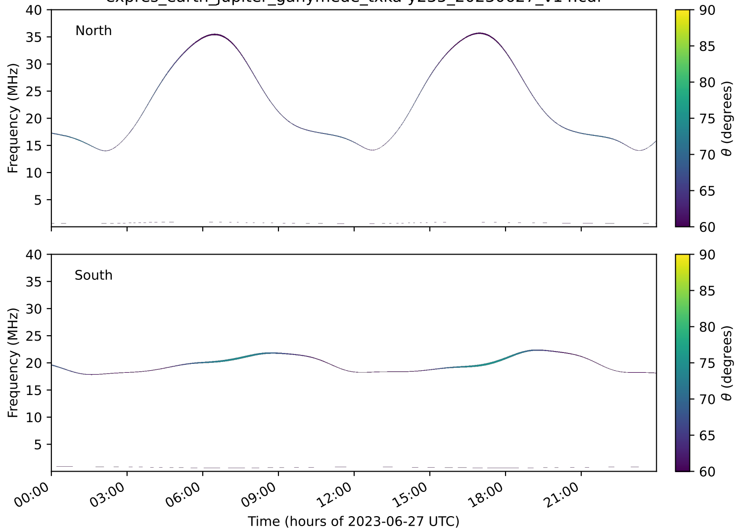
expres_earth_jupiter_ganymede_txka-y235_20230627_v14.cdf
