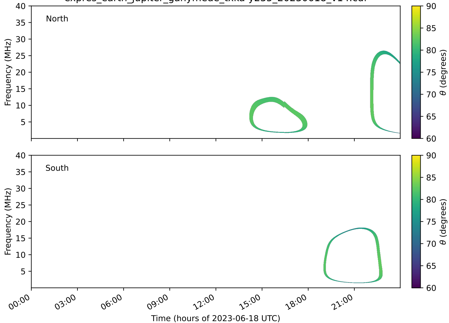
expres_earth_jupiter_ganymede_txka-y235_20230618_v14.cdf
