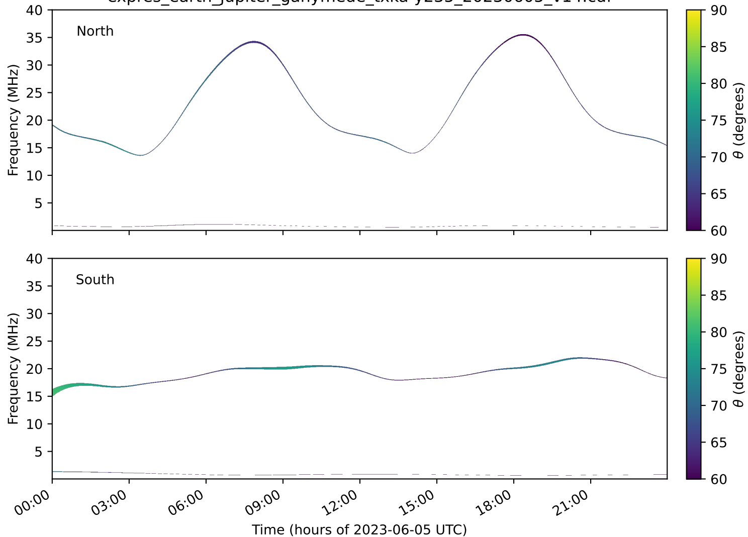
expres_earth_jupiter_ganymede_txka-y235_20230605_v14.cdf
