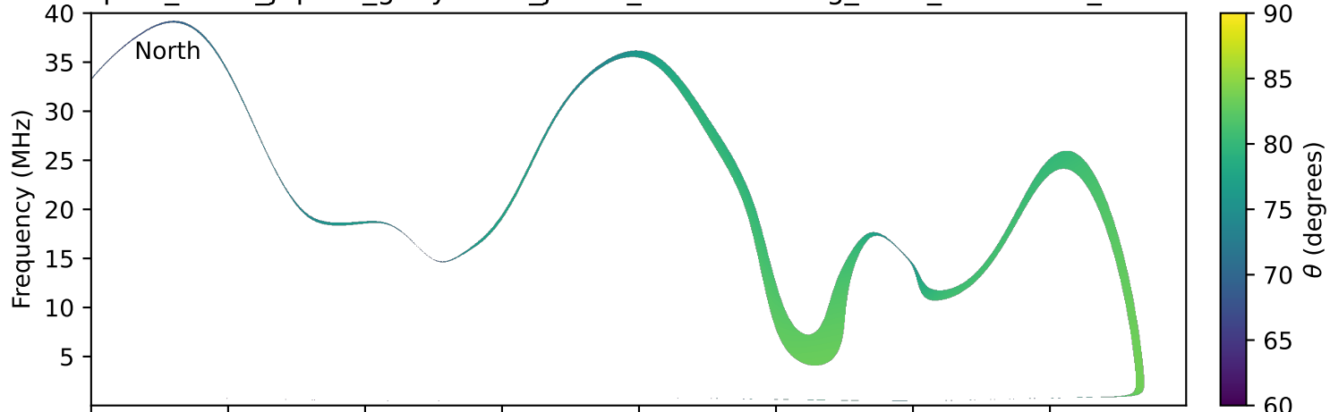
expres_earth_jupiter_ganymede_jrm33_lossc-wid1deg_3kev_20230607_v11.cdf
