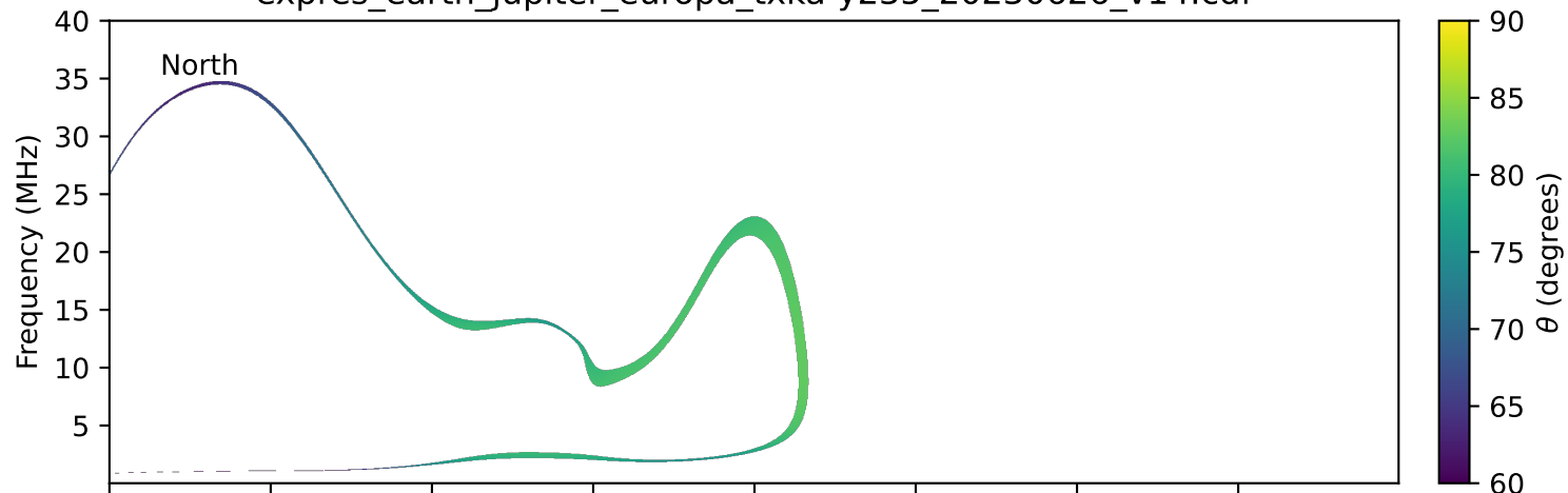
expres_earth_jupiter_europa_txka-y235_20230626_v14.cdf
