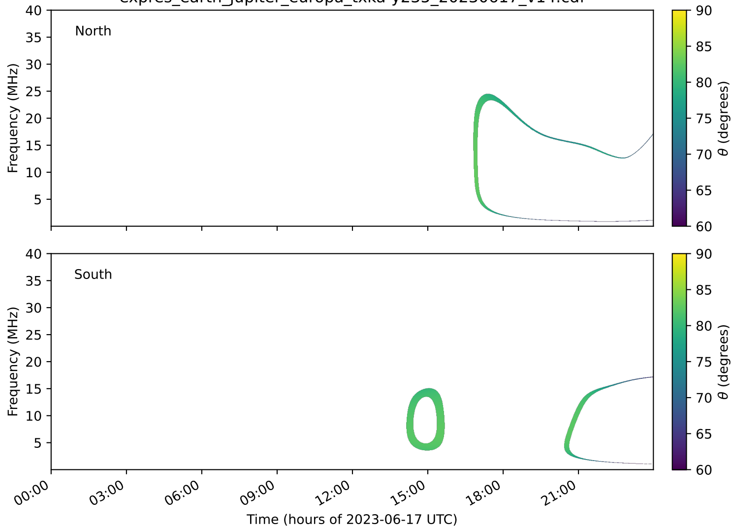
expres_earth_jupiter_europa_txka-y235_20230617_v14.cdf
