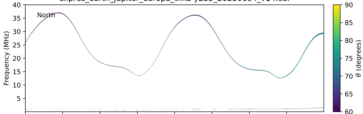
expres_earth_jupiter_europa_txka-y235_20230604_v14.cdf
