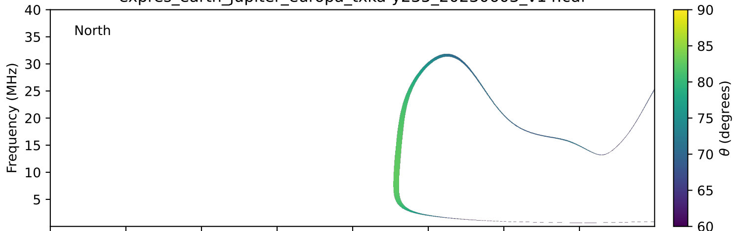
expres_earth_jupiter_europa_txka-y235_20230603_v14.cdf
