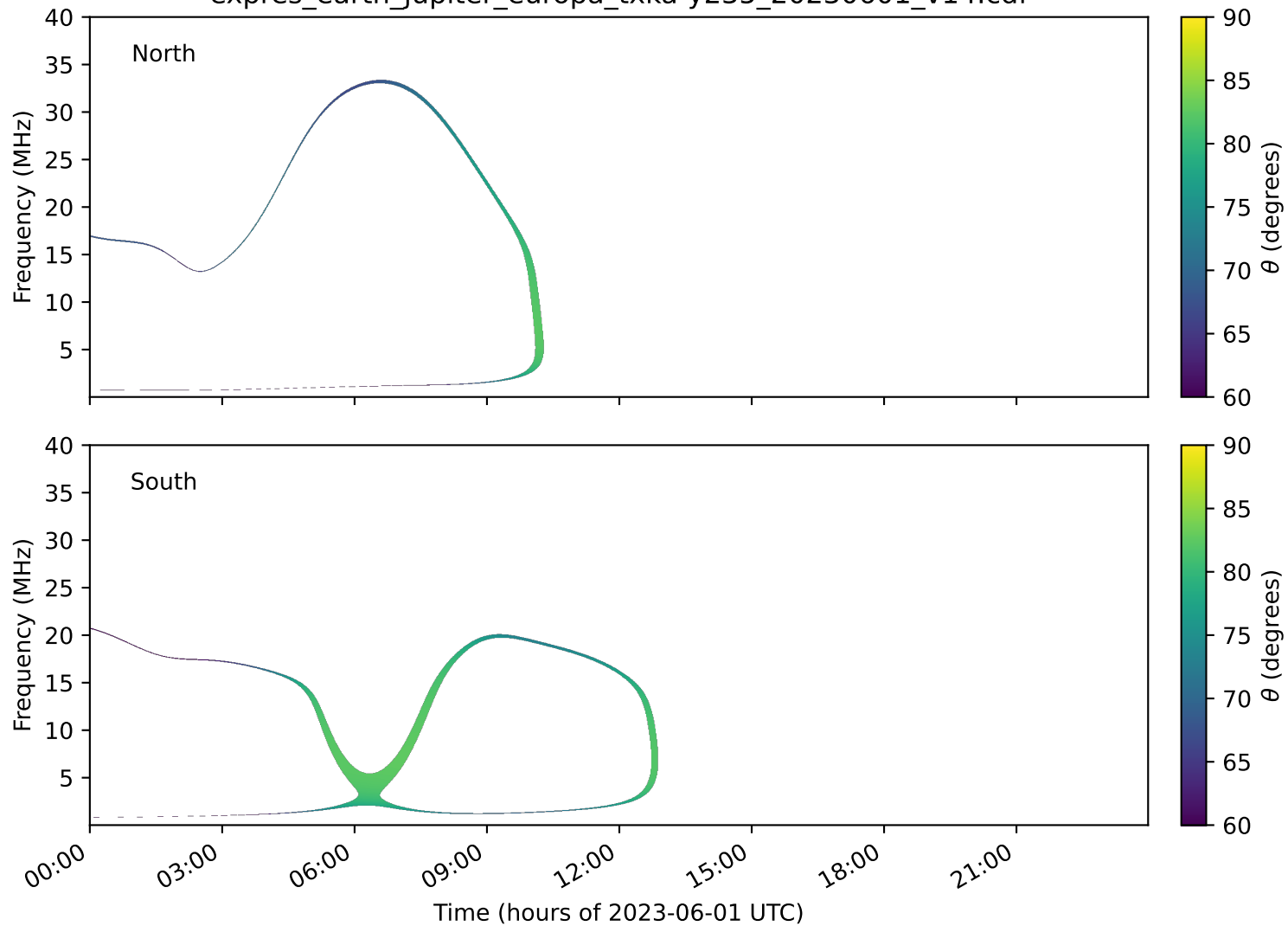
expres_earth_jupiter_europa_txka-y235_20230601_v14.cdf
