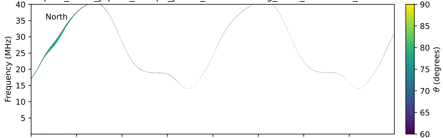
expres_earth_jupiter_europa_jrm33_lossc-wid1deg_3kev_20230625_v11.cdf
