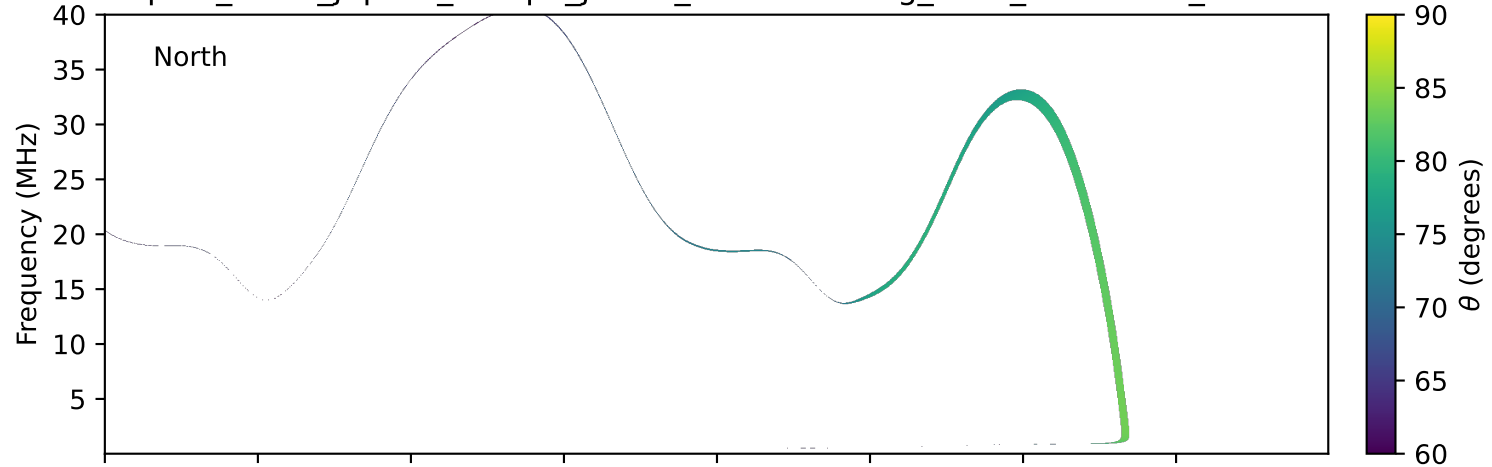
expres_earth_jupiter_europa_jrm33_lossc-wid1deg_3kev_20230615_v11.cdf
