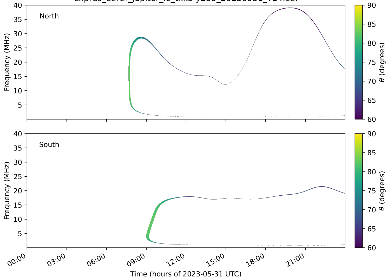
expres_earth_jupiter_io_txka-y235_20230531_v14.cdf
