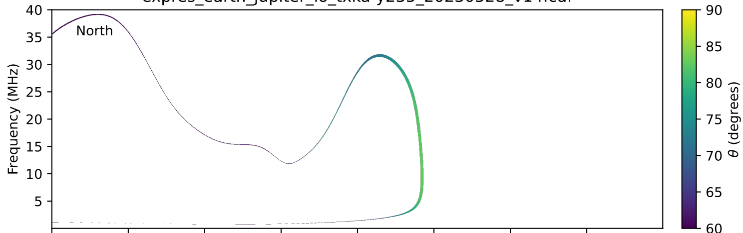
expres_earth_jupiter_io_txka-y235_20230528_v14.cdf
